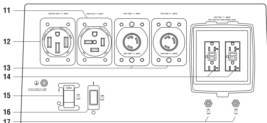
Receptacles and circuit breakers
